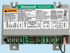
Universal Hot Surface Ignition Control
