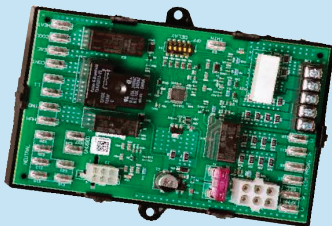
Universal Furnace Fan Timer Board
