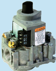
Universal Standard Opening Intermittent Pilot, Hot Surface, or Direct Spark Ignition Valves Nat Or LP Gas
